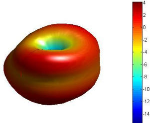
Freq = 0.908GHz Az= 45 EL= 45
