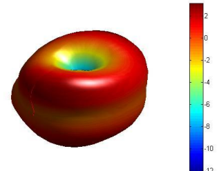
Freq = 0.919GHz Az= 45 EL= 45
